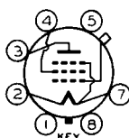
BOTTOM VIEW (GT-5Y)
